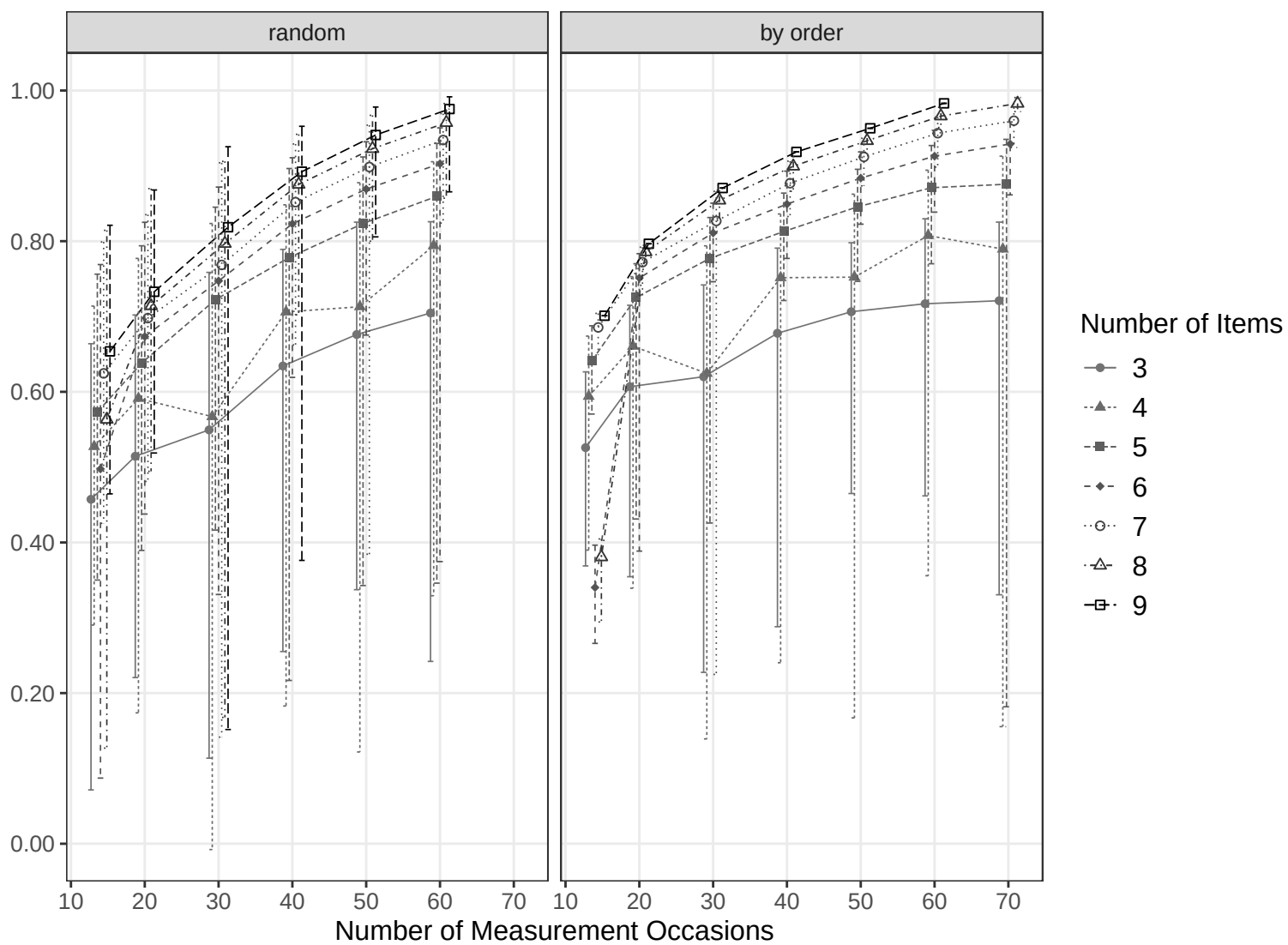
Correlation with Benchmark (ICC.z)
